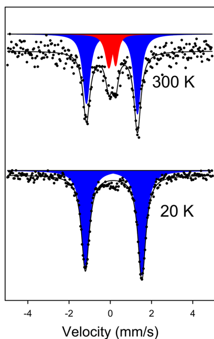
Figure 7. Mössbauer spectra of [\text{Fe}(\text{hapMen})_2]\text{ClO}_4 .
