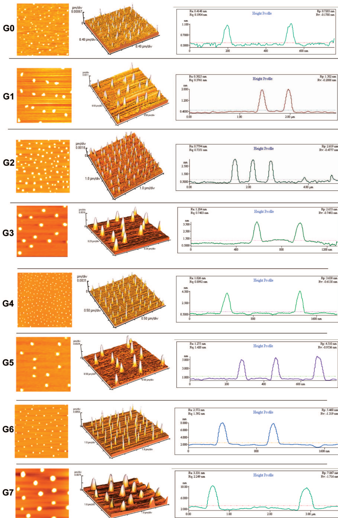
Figure 5. AFM images obtained for the ferrocenyl dendrimers ( G_n -Fc).
