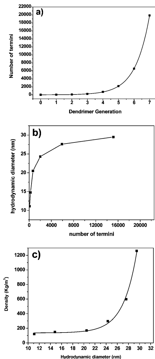
Figure 4. Relationship between the (a) number of termini vs the generation of dendrimer: y = 5.15 + 8.56e^{(x/0.903)} , ( R = 1.00 ); (b) number of termini vs the hydrodynamic diameter; (c) the hydrodynamic diameter vs the density of the dendrimer: y = 136 + 0.00619e^{(x/2.44)} , ( R = 0.996 ).
