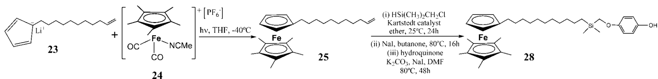
Scheme 4. Synthesis of the Pentamethylferrocenyl Derivative Containing a Long Alkyl Chain and a Phenol Termini.
