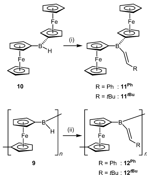
Scheme 5. Hydroboration of PhCCH or t BuCCH with Ferrocenylborane 10 and Polymer 9 a
