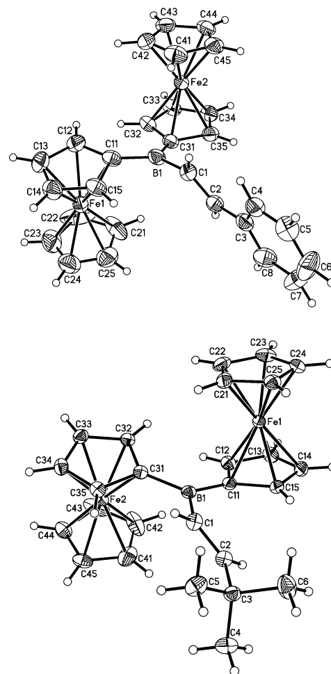
Figure 8. Molecular structures of 11 Ph (top) and 11 tBu (bottom) in the solid state (30% and 50% probability ellipsoids, respectively). Selected bond lengths (Å), bond angles (deg), torsion angles (deg), and dihedral angles (deg) for 11 Ph : B(1)–C(1) 1.575(9), B(1)–C(11) 1.551(7), B(1)–C(31) 1.552(6), C(1)–C(2) 1.340(17); C(1)–B(1)–C(11) 111.5(4), C(1)–B(1)–C(31) 122.4(4), C(11)–B(1)–C(31) 126.0(4), B(1)–C(1)–C(2) 124.3(9), C(1)–C(2)–C(3) 124.2(9); C(2)–C(1)–B(1)–C(11) –123.1(6), C(2)–C(1)–B(1)–C(31) 60.8(7); B(1)C(1)C(2)/C(1)B(1)C(11)C(31) 58.7, C(11) to C(15) ring//C(1)B(1)C(11)C(31) 21.1, C(31) to C(35) ring//C(1)B(1)C(11)C(31) 12.3. For 11 tBu : B(1)–C(1) 1.576(2), B(1)–C(11) 1.562(2), B(1)–C(31) 1.562(2), C(1)–C(2) 1.340(2); C(1)–B(1)–C(11) 120.8(1), C(1)–B(1)–C(31) 116.4(1), C(11)–B(1)–C(31) 122.9(1), B(1)–C(1)–C(2) 126.0(2), C(1)–C(2)–C(3) 129.2(2); C(2)–C(1)–B(1)–C(11) –33.8(2), C(2)–C(1)–B(1)–C(31) 148.2(2); B(1)C(1)C(2)/C(1)B(1)C(11)C(31) 32.7, C(11) to C(15) ring//C(1)B(1)C(11)C(31) 17.2, C(31) to C(35) ring//C(1)B(1)C(11)C(31) 17.1.
