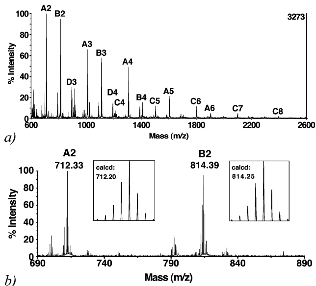
Figure 6. (a) MALDI-TOF mass spectrum of polymer 12 Ph acquired in (+) ion reflector mode. The different series are indicated as A, B, C, and D; the numbers of the individual peaks correspond to the number of repeating units. (b) Expansion of the mass range from 690 to 890 Da and comparison of the peak patterns with those calculated assuming a 10000:1 resolving power.
