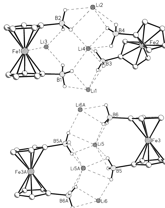
Figure 3. Molecular structure of 4(OEt 2 ) 2,67 in the solid state; hydrogen atoms attached to carbon and Li + -coordinated OEt 2 molecules have been omitted for clarity. (Top) dimer(1); (bottom) dimer(2). Selected bond lengths (Å) and atom⋯atom distances (Å): Dimer(1) B(1)–C(11) 1.586(8), B(2)–C(21) 1.584(8), B(3)–C(31) 1.556(8), B(4)–C(41) 1.579(8), B(1)⋯Li(1) 2.61(1), B(1)⋯Li(3) 2.52(1), B(1)⋯Li(4) 2.67(1), B(2)⋯Li(2) 2.58(1), B(2)⋯Li(3) 2.515(9), B(2)⋯Li(4) 2.68(1), B(3)⋯Li(1) 2.54(1), B(3)⋯Li(4) 2.44(1), B(4)⋯Li(2) 2.48(1), B(4)⋯Li(4) 2.43(1), Fe(1)⋯Li(3) 2.653(9); Dimer(2) B(5)–C(51) 1.579(7), B(6)–C(61) 1.594(7), B(5)⋯Li(5) 2.516(9), B(5)⋯Li(5A) 2.59(1), B(5)⋯Li(6) 2.77(1), B(6)⋯Li(5) 2.51(1), B(6)⋯Li(6A) 2.41(1).
