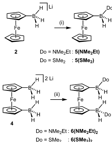
Scheme 2. Synthesis of Mono- and Ditopic Ferrocenylborane Adducts 5 (NMe 2 Et), 5 (SMe 2 ), 6 (NMe 2 Et) 2 , 6 (SMe 2 ) 2 a
