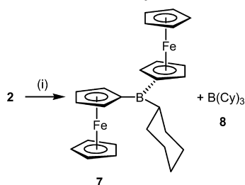
Scheme 3. Preparation of Cyclohexyldi(ferrocenyl)borane 7 and Tricyclohexylborane 8 by Reaction of the Ferrocenylhydridoborate 2 with \text{Me}_3\text{SiCl} in the Presence of Cyclohexene a
