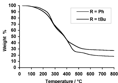
Figure 7. Thermogravimetric analysis plots of 12 Ph and 12 tBu .
