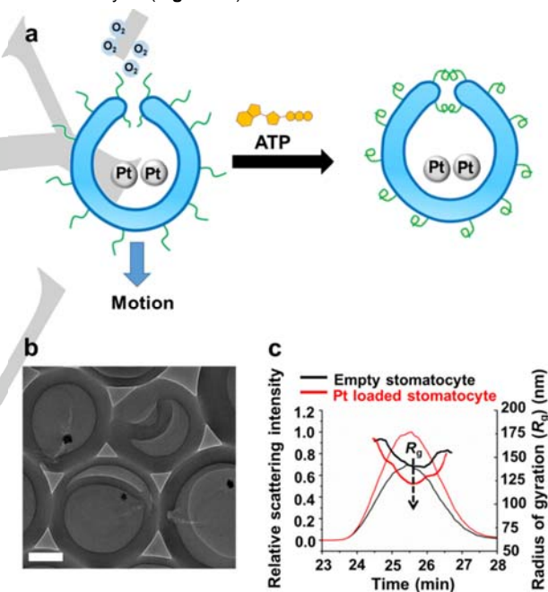
Figure 4. (a) Schematic representation of ATP-regulated PtNP loaded stomatocyte nanomotors. (b) TEM image of PtNP loaded PLL-stomatocytes. Scale bar represents 100 nm. (c) Asymmetric flow field-flow fractionation (AF4) fractograms and radius of gyration ( R_g ) of empty PLL-stomatocytes and PtNP loaded PLL-stomatocytes.
