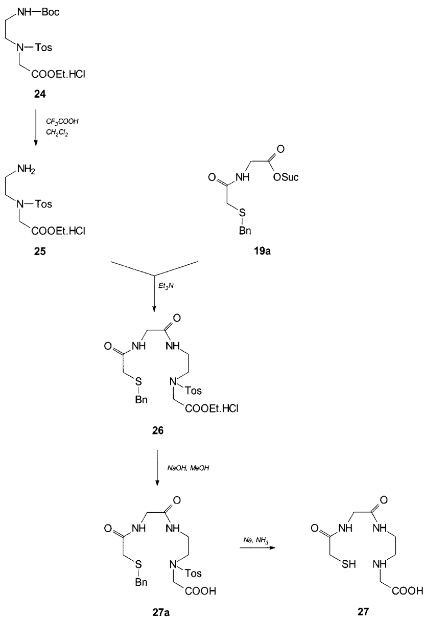
Scheme 6. Continued.
