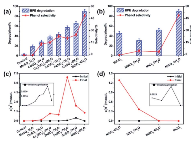
Fig. 1 (a and b) Effect of transition metal salts on BPE degradation efficiency and phenol selectivity. Condition: 300 mg BPE, 1.4 mmol transition metal salts, 20 mL methanol, 200\text{ }^\circ\text{C} , 5 h. (c and d) Hydrogen ion concentration ( c(H^+) ) of catalyst systems. Condition: 1.4 mmol transition metal salts, 20 mL methanol, 200\text{ }^\circ\text{C} , 5 h.
