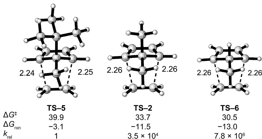
Fig. 5. Transition state structures and Gibbs free activation ( \Delta G^\ddagger ) and reaction ( \Delta G_{\text{rxn}} ) energies in kcal/mol for the Diels–Alder reactions of 5-methyl-5- t -butyl-cyclopentadiene (TS-5), 5,5-dimethylcyclopentadiene (TS-2), and 5-methylcyclopentadiene (TS-6) with ethylene.
