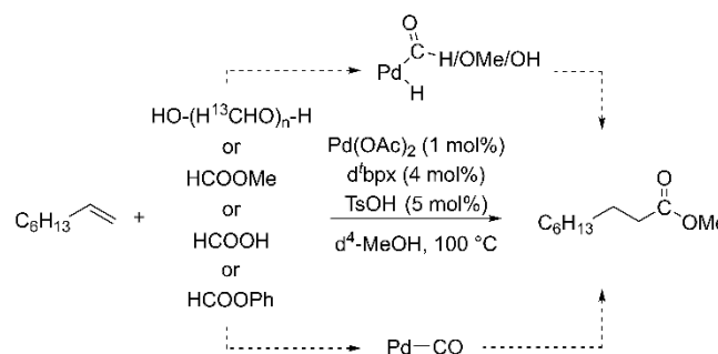
Scheme 1. The model reaction studied in this work: Pd-catalyzed alkoxy carbonylation of 1-octene with 13 C-PFA, methyl formate, formic acid or phenyl formate in d 4 -MeOH.
