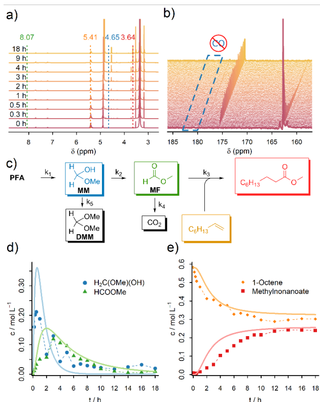
Figure 1. a) Selected ex-situ ^1\text{H} NMR spectra measured in d^4 -MeOH. b) Selected in-situ ^{13}\text{C} NMR spectra in the carbonyl region. Importantly no CO signal (181 - 185 ppm [16] ) is observed. c) Scheme illustrating the species considered for the microkinetic model, their possible reaction pathways and the respective kinetic rate constants. d-e) Data points and kinetic fits of MM (blue), MF (green), 1-octene (orange) and methyl nonanoate (red) based on the time-dependent concentrations extracted from ex-situ ^1\text{H} NMR spectra (signals annotated in a)).
