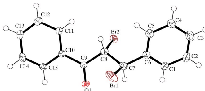
Figure 1 A view of (I), showing 50% probability displacement ellipsoids; H atoms are shown as arbitrary spheres.
