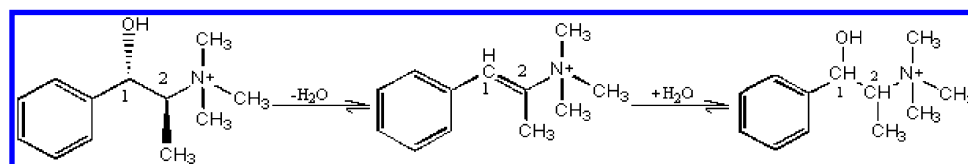
Figure 2. Structure of (1 S ,2 R )-(+)- N,N -dimethylephedrinium ion, its achiral dehydration product, and racemic nature upon addition of water.
