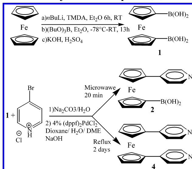
Scheme 1. Synthesis of Complexes 1, 2, and 4
