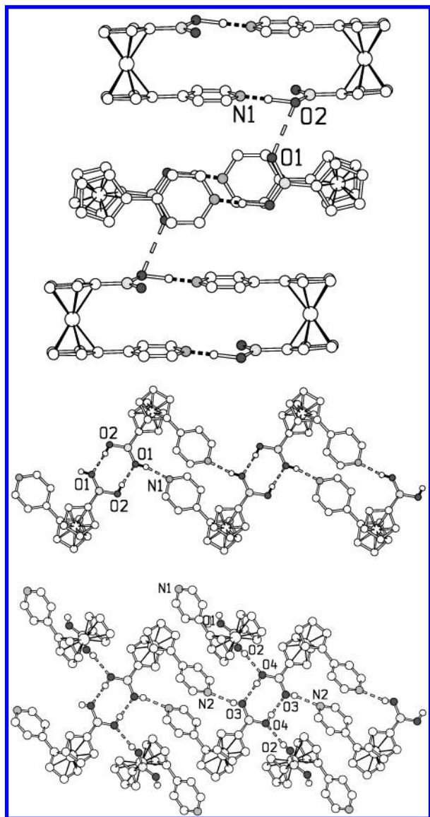
Figure 2. (a, top) Hydrogen-bonded dimers formed by (B)-OH \cdots N interactions in crystalline 2a . Note how the dimers are connected via (B)OH \cdots O(B) interactions. The H atom bound to O(1) was not observed (see the Experimental Section). (b, middle) Hydrogen-bonding pattern in crystalline 2b . Note how the ligand conformation has changed from eclipsed in 2a to cisoid in 2b . (c) Hydrogen-bonding pattern in crystalline 2c . Note the similarity of the ligand conformation to that in 2b and the presence of lateral (B)-OH \cdots O(B) interactions as in 2a . H CH atoms are not shown for clarity.
