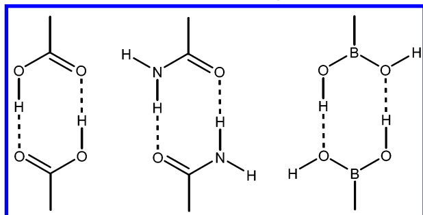
Chart 1. Comparison between Hydrogen-Bonding Ring Motifs Involving Carboxylic (Left), Amido (Middle), and Boronic (Right) Groups
