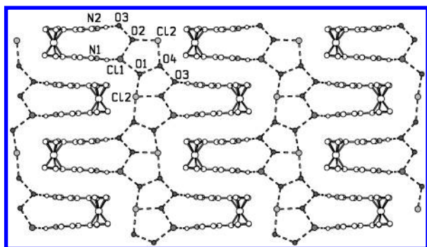
Figure 5. Formation of hydrogen-bonding interactions of the ^+\text{N}-\text{H}\cdots\text{O}_{\text{water}} and of the ^+\text{N}-\text{H}\cdots\text{Cl}^- type by the \text{N}-\text{H} donors on each complex in crystalline 5 . The cations are arranged in piles and are connected to cations on adjacent piles via a network of \text{O}(\text{H})_{\text{water}}\cdots\text{O}_{\text{water}} and \text{O}(\text{H})_{\text{water}}\cdots\text{Cl}^- hydrogen-bonding interactions.
