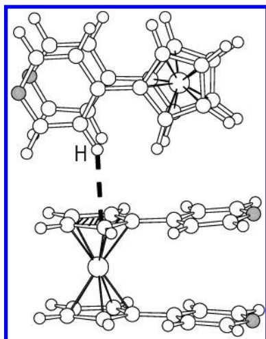
Figure 4. \text{CH}\cdots\pi interaction ( (\text{C})\text{H}\cdots\pi = 2.66 \text{ \AA} , \text{C}-\text{H}\cdots\pi = 146.3^\circ ) observed in crystalline 4 . The broken line represents the distance from the H atom to the plane of the aromatic ring on the adjacent molecule.
