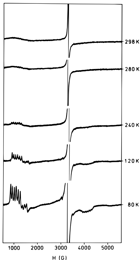
Figure 7. Selected X-band powder EPR spectra of Mn(II)-doped [\text{Fe}(\text{abpt})_2(\text{TCNQ})_2] .
