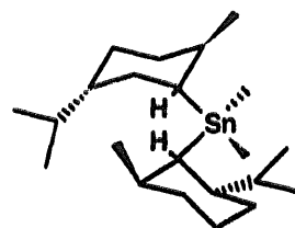
Fig. 1. Di(-)-menthildimethyltin 1 .
