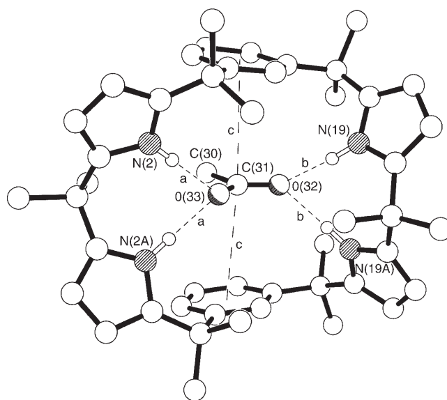
Figure 7. Molecular structure of the C_2 -symmetric macrocycle and encapsulated anion present in the crystals of m -6 \cdot\text{CH}_3\text{COO}^- . Hydrogen-bonding geometries \text{N}\cdots\text{O} , \text{H}\cdots\text{O}[\text{Å}] and \text{N}-\text{H}\cdots\text{O}[\text{Å}] , respectively, are a) 2.805(3), 1.91, 1.78; b) 2.764(3), 1.87, 1.73, and the \pi - \pi interactions (c) have mean interplanar and centroid \cdots\text{C}(31) separations of \approx 3.55 and 3.58\text{ Å} , respectively (aryl and acetyl planes are inclined by \approx 7^\circ ).
