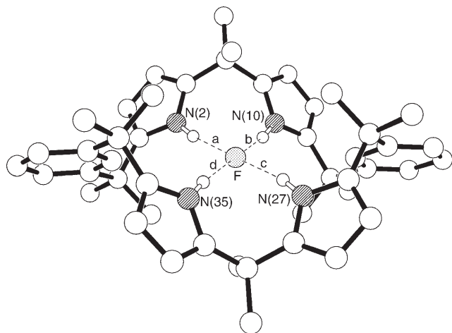
Figure 4. Molecular structure of one ( I ) of the two independent “macrocycle and encapsulated anion” complexes present in the crystals of m - 6 ·F − . Hydrogen-bonding geometries N⋯F, H⋯F[Å] and N–H⋯F[°], respectively, are: a) 2.917(3), 2.03, 170; b) 2.922(4), 2.04, 166; c) 2.890(3), 2.00, 169; d) 2.918(3), 2.03, 171.
