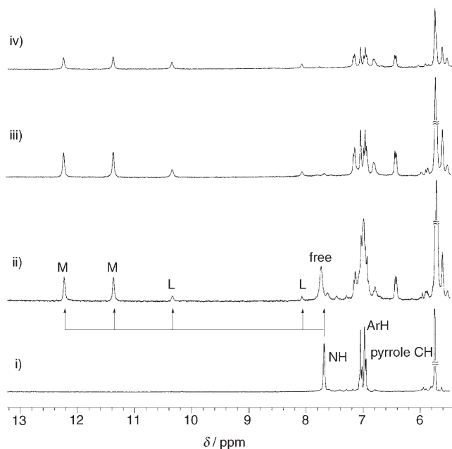
Figure 6. CIS in ^1\text{H} NMR spectra of m -6 upon addition of \text{CH}_3\text{COONBu}_4\text{N} at −30°C: i)–iv) 0, 0.5, 1.2 and 2.5 equivalents of added salt, respectively; each pair of M and L resonances always have 1:1 intensities, the M:L ratios in ii)–iv) are 3.8, 2.1 and 1.3, respectively.
