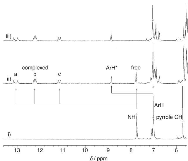
Figure 3. ^1H NMR spectra ( CD_2Cl_2 , -65^\circ C ) of: i) m-6 , 0.005 M, ii) m-6 + nBu_4NF (1:0.77) and iii) m-6 + nBu_4NF (1:1.81). The intensities and J(H,F) of the NH resonances of the complex (a, b and c) are 1:2:1 and 52, 22 and 27 Hz, respectively. ArH^* accounts for only one of the “isolated” ArH protons of the complex. No free m-6 is visible in iii).
