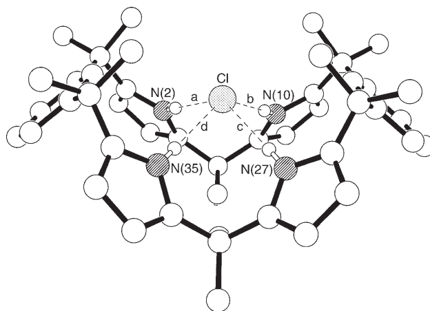
Figure 5. Molecular structure of the macrocycle and the encapsulated anion present in the crystals of m - 6 ·Cl − . Hydrogen-bonding geometries N⋯Cl, H⋯Cl[Å] and N–H⋯Cl[°], respectively, are a) 3.3816(15), 2.49, 172; b) 3.3254(14), 2.43, 173; c) 3.4216(14), 2.52, 178; d) 3.4241(14), 2.53, 174.
