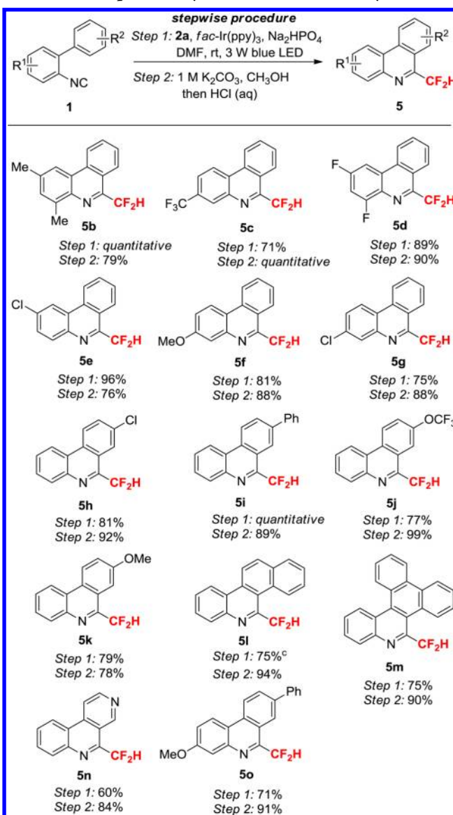
Scheme 2. Scope of Isocyanides of Difluoromethylation a,b
