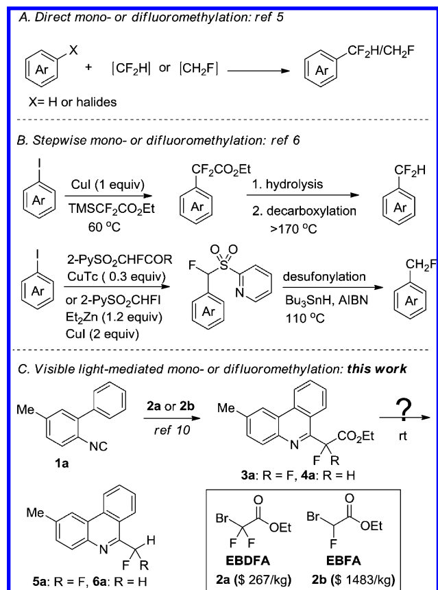
Figure 1. Major strategies of mono- and difluoromethylation of arenes.
