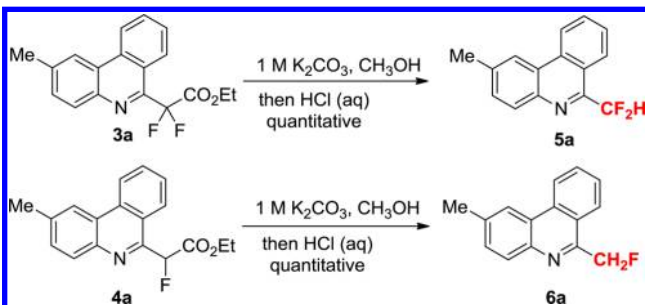
Scheme 1. Room Temperature Decarboxylation
