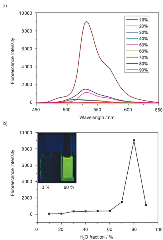
Figure 1. a) Fluorescence spectra of 2,2-dihydroxy-1,1-naphthalazine (10 \mu\text{M} , \lambda_{\text{ex}} = 400 nm) in THF/water with different water percentages. b) Plot of maximum fluorescence intensity vs. % water. Inset: image of 2,2-dihydroxy-1,1-naphthalazine in THF/water mixtures with 0% (left) and 80% water (right) under UV illumination at 365 nm.
