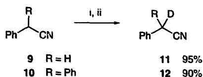
Scheme 3. Reagents: (i) \text{PhMe}_2\text{SiLi} , THF, 0 °C, 30 min; (ii) AcOD, 0 °C; (iii) HCl, \text{H}_2\text{O} , r.t., 30 min.
