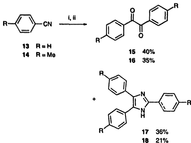
Scheme 4. Reagents: (i) \text{PhMe}_2\text{SiLi} , THF, 0 °C, 2 h; (ii) HCl, \text{H}_2\text{O} , reflux, 2 h.
