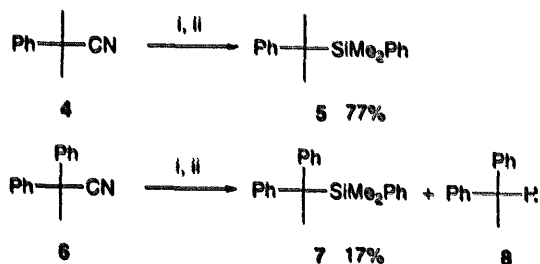
Scheme 2. Reagents: (i) \text{PhMe}_2\text{SiLi} , THF, 0 °C, 4 h; (ii) HCl, \text{H}_2\text{O} , r.t., 1 h.
