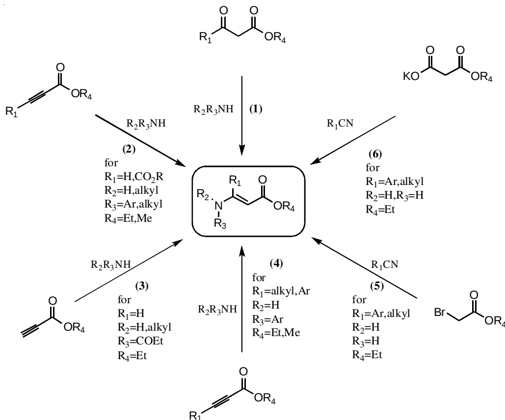
Scheme-I: Synthesis of b-enamino esters
