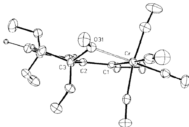
Fig. 4. "Side-on" view of XIX showing the distortions from planarity of the quinone-bisketal ring induced by the coordination of one methoxy group to the metal center.
