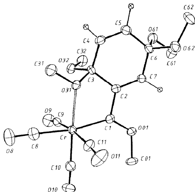
Fig. 3. Molecular structure of XIX (without methyl hydrogens).
