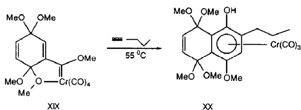
Scheme 10
