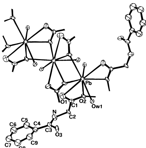
Figure 6. ORTEP view of the Pb atom environment in [\text{Pb}(\text{bzgly}-\text{O})_2(\text{H}_2\text{O})_2] \cdot 2\text{H}_2\text{O} ( 2 ) with the atom-numbering scheme.
