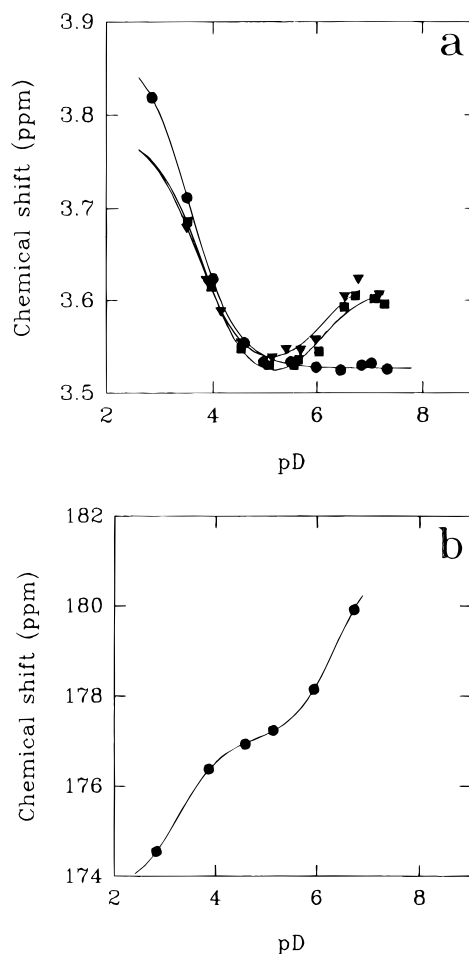
Figure 2. (a) pD dependence of the chemical shift of the methylene resonance in the ^1H NMR spectrum of tsgly in D_2O : (●) free ligand; (▼) saturated solution of [Pb(tsgly-N,O)(H_2O)] (1); (■) saturated solution of 1 plus bpy in a 1:1 molar ratio with the metal. T = 300 K. [Pb^{2+}] = 2 \times 10^{-3} M. (b) pD dependence of the chemical shift of the ^{13}C NMR resonance of the isotopically enriched carboxylic carbon of tsgly in the presence of the Pb^{2+} ion in a 2:1 ligand-to-metal molar ratio. T = 300 K. [Pb^{2+}] = 1 \times 10^{-3} M.
