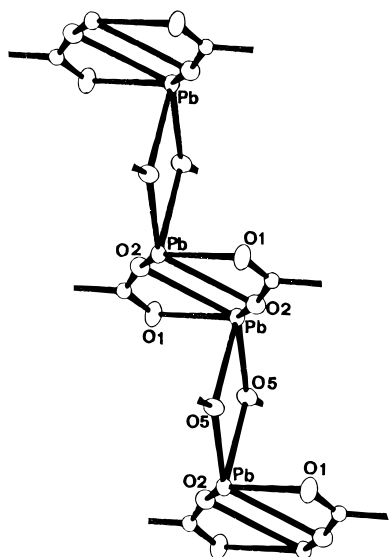
Figure 8. Arrangement of the polymeric square-planar \text{Pb}_2\text{O}_2 rings in 3 .
