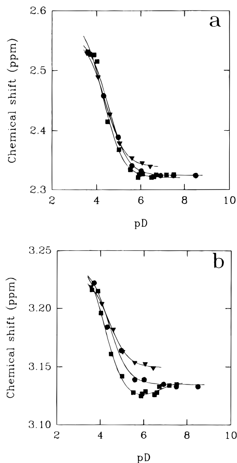
Figure 4. pD dependence of the chemical shift of the central peak of the two methylene triplets in the ^1\text{H} NMR spectrum of \text{ts}\beta\text{ala} in \text{D}_2\text{O} : (a) \alpha\text{-CH}_2 ; (b) \beta\text{-CH}_2 ; (●) free ligand; (▼) saturated solution of the crystalline compound [\text{Pb}(\text{ts}\beta\text{ala-O})_2]\cdot\text{H}_2\text{O} ; (■) saturated solution of the crystalline compound [\text{Pb}(\text{ts}\beta\text{ala-O})_2]\cdot\text{H}_2\text{O} plus \text{bpy} in a 1:1 molar ratio with the metal. T = 300\text{ K} . [\text{Pb}^{2+}] = 1 \times 10^{-3}\text{ M} .
