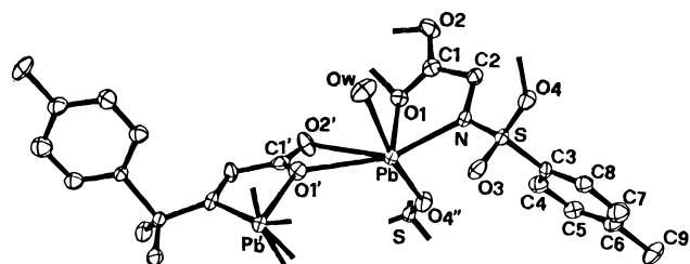
Figure 5. ORTEP view of the Pb atom environment in [\text{Pb}(\text{tsgly-N,O})(\text{H}_2\text{O})] (1) with the atom-numbering scheme.
