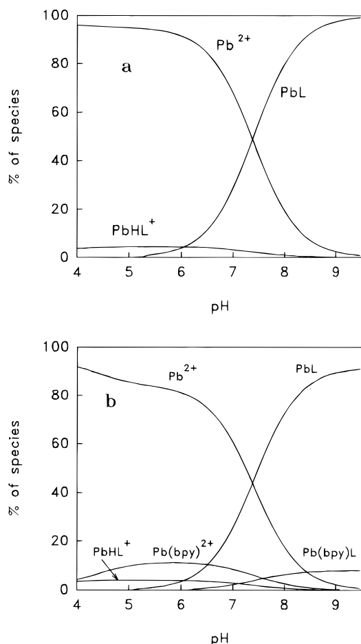
Figure 1. Species distribution curves for (a) the binary Pb-tsgly system and (b) the ternary Pb-tsgly-bpy system, with molar ratios of 1:20 and 1:20:1, respectively. [Pb^{2+}] = 2 \times 10^{-4} M.
