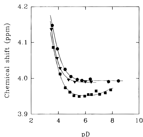
Figure 3. pD dependence of the chemical shift of the methylene resonance in the ^1H NMR spectrum of bzgly in D_2O : (●) free ligand; (▼) saturated solution of [Pb(bzgly-O)_2(H_2O)_2 \cdot 2H_2O] (2); (■) saturated solution of 2 plus bpy in a 1:1 molar ratio with the metal. T = 300 K. [Pb^{2+}] = 1 \times 10^{-3} M.
