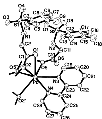
Figure 7. ORTEP view of the Pb atom environment in [Pb(tsgly-O) 2 -(bpy)] ( 3 ) with the atom-numbering scheme.
