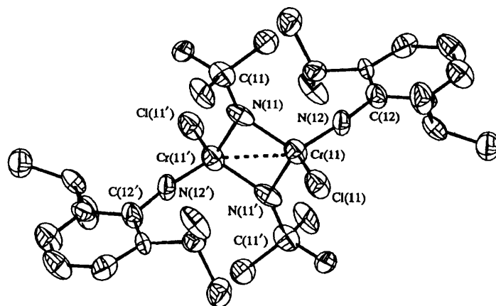
Fig. 3 Structure of the chromium(v) dimer [\text{CrCl}(\mu\text{-NBu}')(\text{NC}_6\text{H}_3\text{Pr}_2\text{-2,6})]_2 \mathbf{3}
