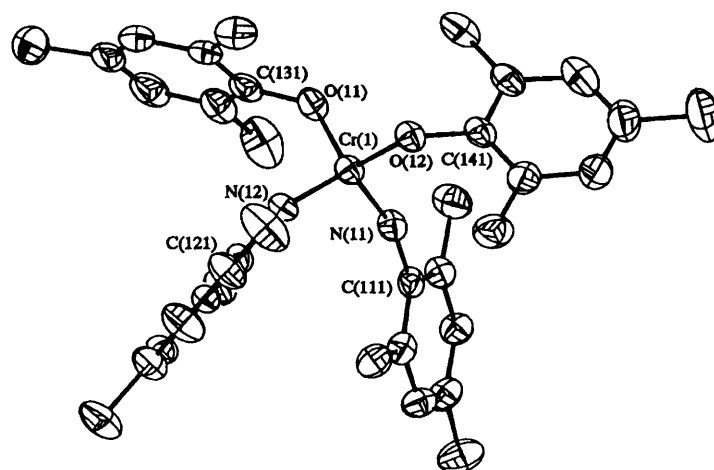
Fig. 4 Co-ordination sphere of \text{Cr}(\text{NC}_6\text{H}_2\text{Me}_3\text{-2,4,6})_2(\text{OC}_6\text{H}_2\text{Me}_3\text{-2,4,6})_2 \cdot 0.25\text{Et}_2\text{O} 7
