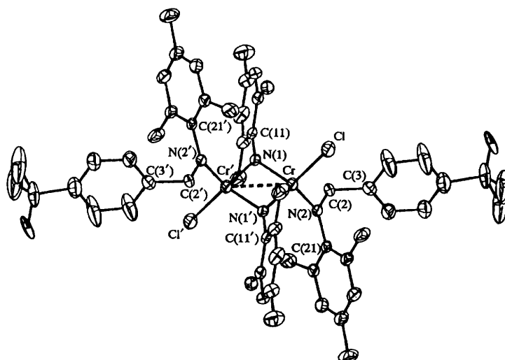
Fig. 5 Co-ordination sphere of \{\text{CrCl}(\mu\text{-NC}_6\text{H}_4\text{Me}_3\text{-2,4,6})[\text{N}(\text{CH}_2\text{C}_6\text{H}_4\text{Bu}^t\text{-4})(\text{C}_6\text{H}_2\text{Me}_3\text{-2,4,6})]\}_2\cdot 2\text{Et}_2\text{O} 14 . One conformation of the disordered tert -butyl group is shown
