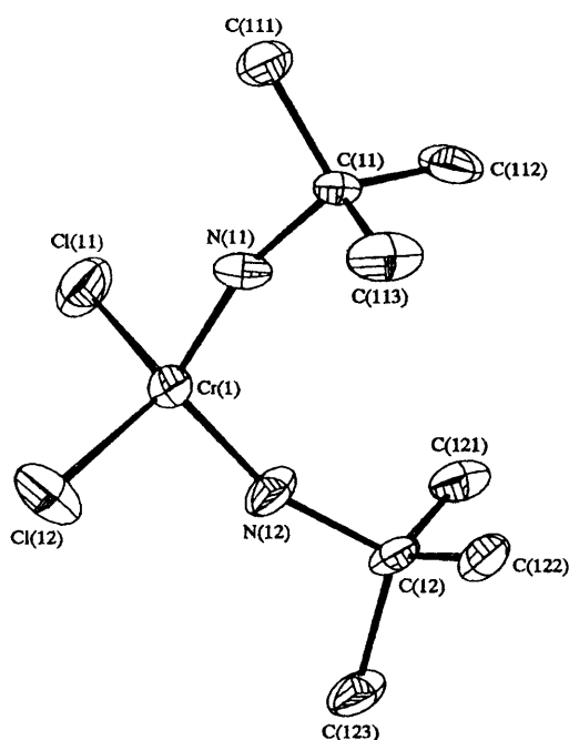
Fig. 2 Structure of \text{CrCl}_2(\text{NBu}^t)_2 1a
