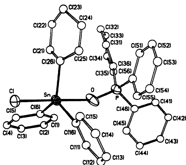
Fig. 1. ORTEP drawing and labeling scheme for 1. Ellipsoids are drawn at 35% probability. Hydrogen atoms are omitted and carbon atoms are set at a fixed radius for clarity.
