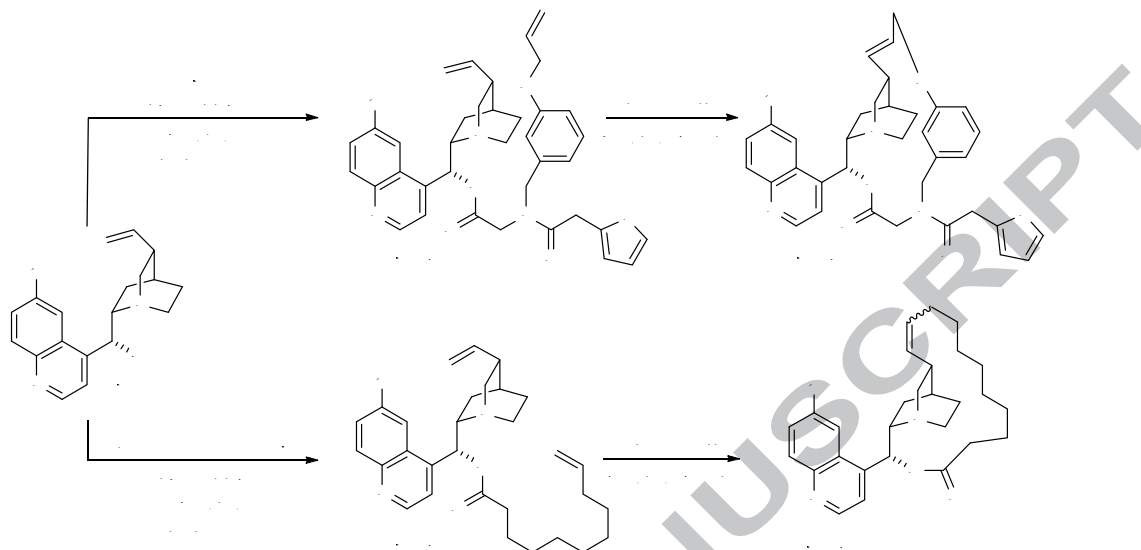
Scheme 8: Synthesis of macrocycles 12 and 13
