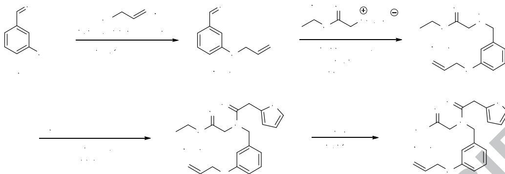
Scheme 5: Synthesis of building block 18
