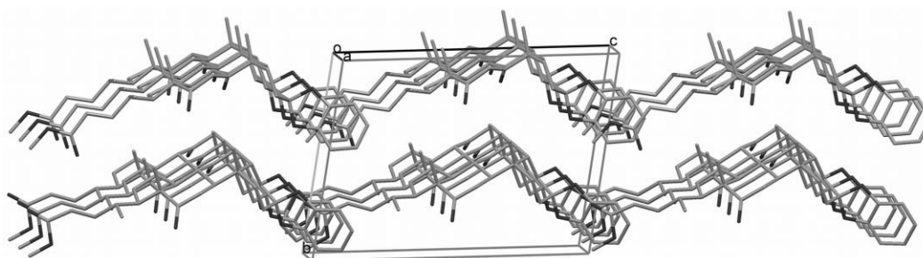
Fig. 8 Packing in the crystal of 7c . The disorder in the side chain and the hydrogen atoms are omitted for clarity.
