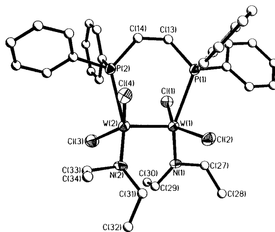
Figure 12. Perspective drawing of trans,trans -W 2 Cl 4 (NEt 2 ) 2 (dppe) ( 8 ). Atoms are represented by thermal ellipsoids at the 40% probability level. Carbon atoms are shown as spheres of arbitrary radii. Phenyl rings are not labeled for clarity.
