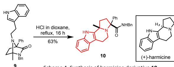
Scheme 4. Synthesis of harmicine derivative 10
