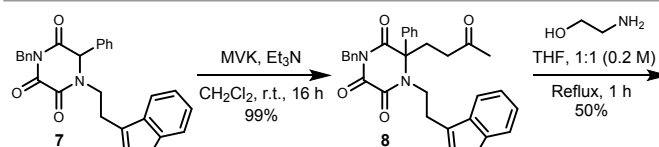
Scheme 3. Reaction pathway to prolinamides 5a+b a) L-selectride, 1.0:1.3 dr; b) LiAlH 4 , 1.5:1.0 dr
