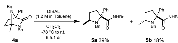
Scheme 2. Reductive ring opening of 4a
