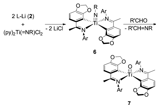
Scheme 5. Synthesis of the Titanium Imido Derivative 6 and Its Subsequent Reactivity with Aldehydes To Form the Analogous Oxo Product 7 a
