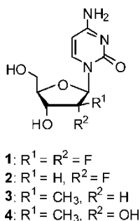
Figure 1: Structures of several 2'-modified nucleosides.
