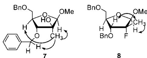
Figure 2: ^1\text{H} NMR NOE correlations of compounds 7 and 8 .
