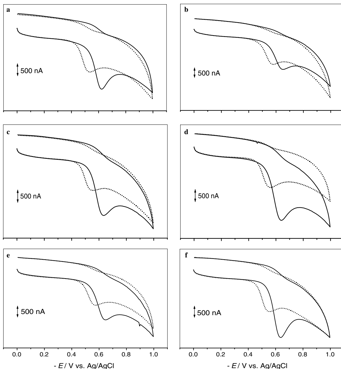
Figure 3. Cyclic voltammograms for several \beta -nitrostyrene ( \cdots ) and \beta -methyl- \beta -nitrostyrene derivatives ( — ), in 100 \mu M solution, at physiological pH. (a) Ia , Ib ; (b) IIa , IIb ; (c) IIIa , IIIb ; (d) IVa , IVb ; (e) Va , Vb ; (f) VIa , VIb . Scan rate 75 mV s -1 .
