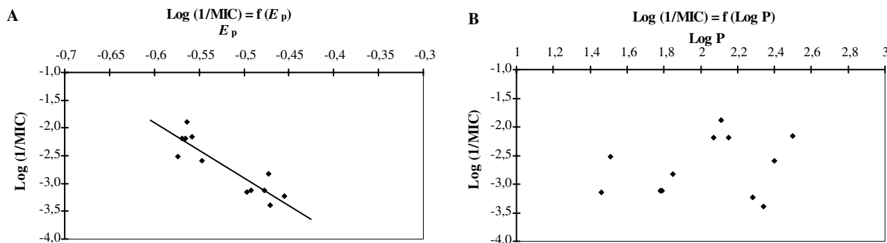
Figure 5. Regression plots of \log(1/\text{MIC}) towards Enterococcus faecalis ATCC 29212, for the \beta -nitrostyrene derivatives tested: (A) standard redox potential values at physiological pH; (B) \log P values.
