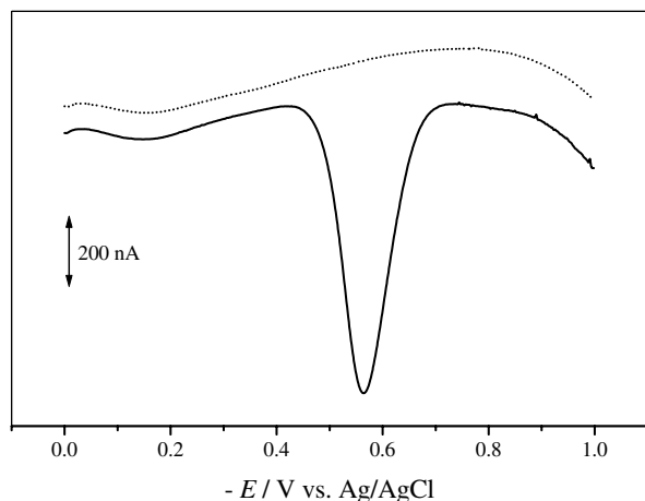
Figure 2. Differential pulse voltammogram for reduction of VIb , in pH 7.3 supporting electrolyte, in the absence (·····) and presence (—) of 100 \mu M VIb . Scan rate 5 \text{mV s}^{-1} .
