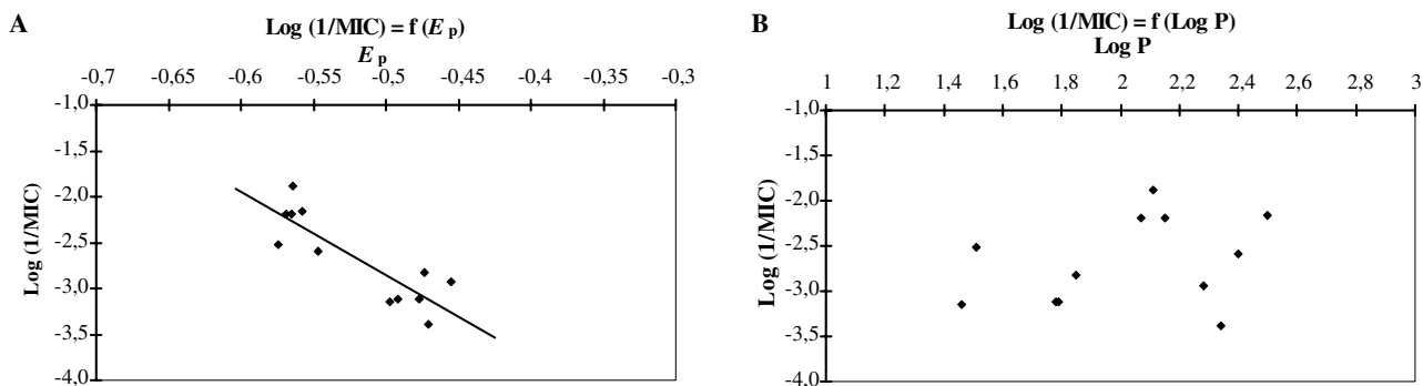
Figure 4. Regression plots of \log(1/\text{MIC}) towards Staphylococcus aureus ATCC 29213, for the \beta -nitrostyrene derivatives tested: (A) standard redox potential values at physiological pH; (B) \log P values.
