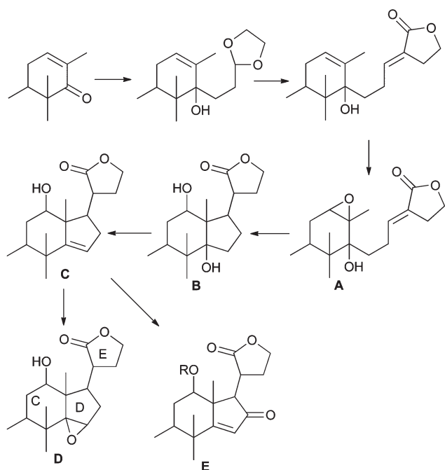
Scheme 2 C-12 Oxygenated CDE limonoid fragment synthetic plan.
