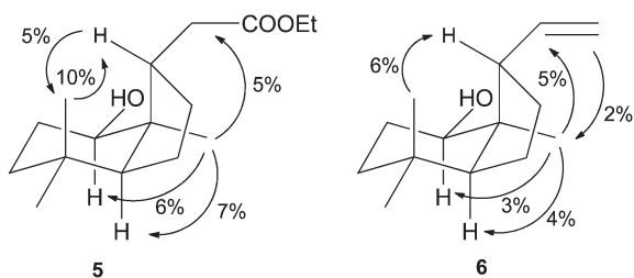
Fig. 2 NOE values of compounds 5 and 6.
