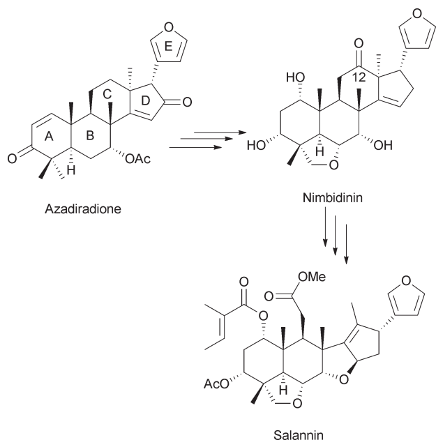
Scheme 1 Limonoid biogenetic relationship.
