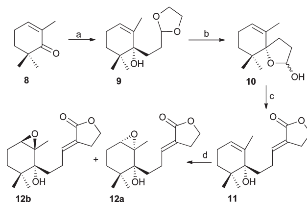
Scheme 6 Reagents and conditions: (a) 2-(2-bromoethyl)-1,3-dioxolane, Li, THF, 65%. (b) AcOH–THF–H 2 O, reflux, 100%. (c) \gamma -butyrolactonyl triphenyl phosphorane, DME, 41%. (d) m -CPBA, CH 2 Cl 2 , 89%.
