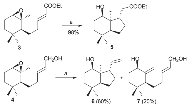
Scheme 4 Reagents and conditions: (a) \text{Cp}_2\text{TiCl}_2 , THF, 25 °C.
