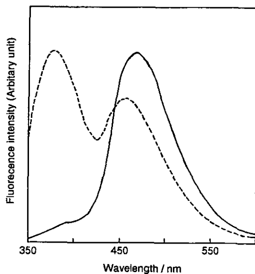
Figure 2. Fluorescence spectra of 3-phenyl-2,4(1 H ,3 H )-pteridinedione ( 3a ): in EtOH (—), in MeCN (---); excitation wavelength=320 nm.
