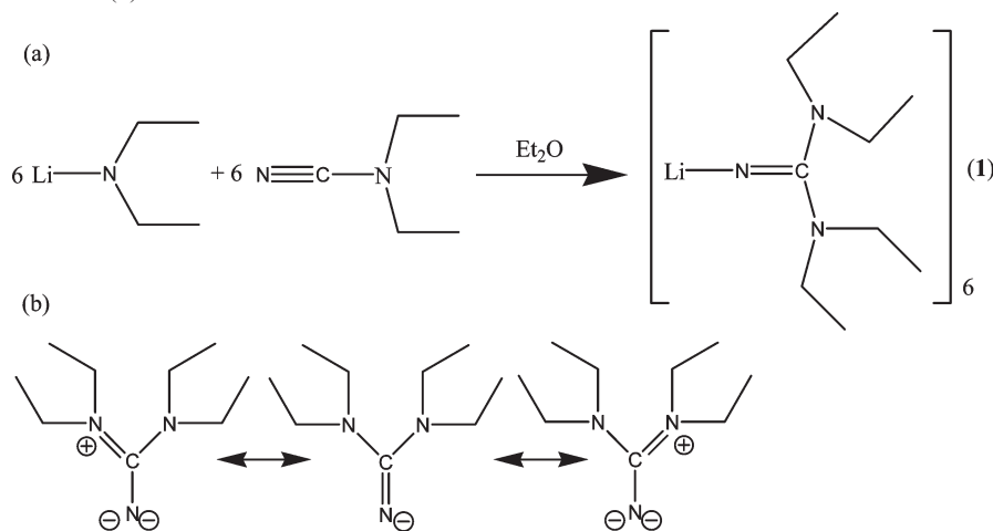
Scheme 1. (a) Synthesis of 1 and (b) the Zwitterionic Resonance of the TEG Anion
