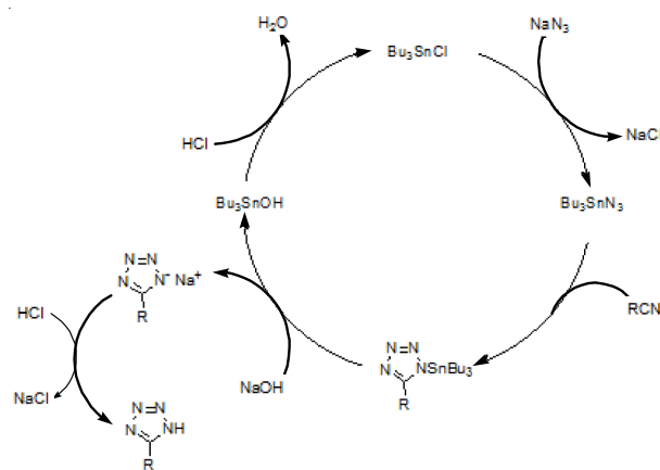
Fig. 2. Cyclic pathway of recycle and reuse of tributyltin chloride
