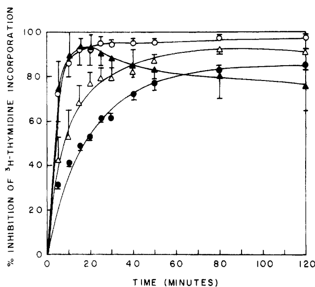
Figure 3. Cytotoxicity of 5,6-DHT's toward differentiated N-2a cells as a function of time. The cells were incubated for up to 120 min with either 5,6-DHT (500 \mu M; \Delta ), 4-Me-5,6-DHT (16a, 500 \mu M; \circ ), 7-Me-5,6-DHT (16b, 500 \mu M; \bullet ), or 4,7-Me 2 -5,6-DHT (16c, 10 \mu M; \blacktriangle ). For details see the Experimental Section. The bars denote mean \pm SD of at least three independent measurements in duplicate.
