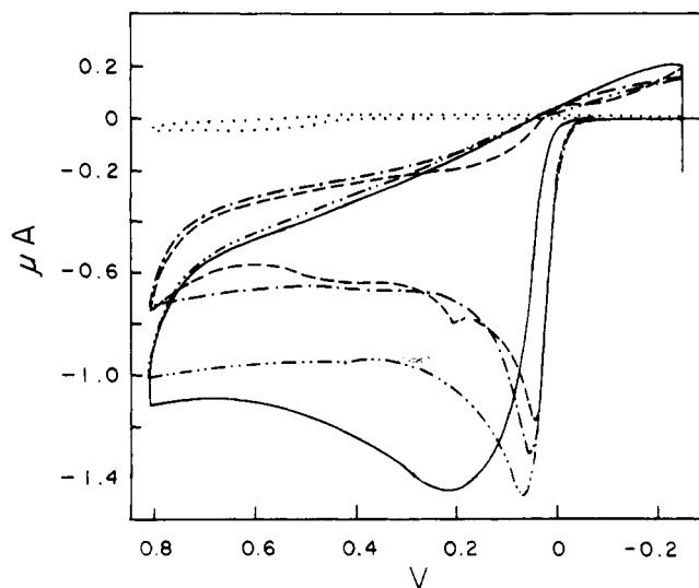
Figure 1. Cyclic voltammograms of 5,6-DHT and its methylated analogues in phosphate buffer containing 0.9% NaCl at pH 7.2 at a scan rate of 50 mV/s: —, 5,6-DHT; ---, 4-Me-5,6-DHT ( 16a ); - - -, 7-Me-5,6-DHT ( 16b ); ···, 4,7-Me 2 -5,6-DHT ( 16c ); ···, background.
