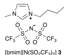
Figure 1. The ionic liquid 1-butyl-3-methylimidazolium bis(trifluoromethanesulfonyl)imide ([bmim][N(SO 2 CF 3 ) 2 ], 3 ) used in this study.
