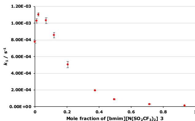
Figure 2. The dependence of the unimolecular rate constant ( k_1 ) of the reaction of the acetobromogalactose 1 on the mole fraction of [bmim][N(SO 2 CF 3 ) 2 ] 3 (♦) in methanol at 315 K. Uncertainties reported are the standard deviation of triplicate measurements; some uncertainties fall within the size of the markers used.
