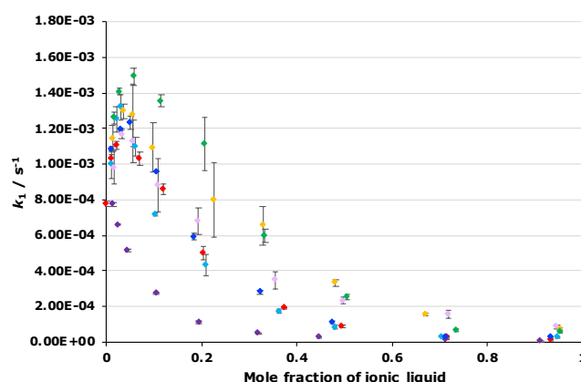
Figure 4. The dependence of the unimolecular rate constant ( k_1 ) of the reaction of the acetobromogalactose 1 on the mole fraction of on the mole fraction of either [bmim][N(SO 2 CF 3 ) 2 ] 3 (♦), [bmim][N(SO 2 CF 3 ) 2 ] 4 (◆), [bmim][N(SO 2 CF 3 ) 2 ] 5 (◆), [mtoa][N(SO 2 CF 3 ) 2 ] 6 (◆), [bmim][PF 6 ] 7 (◆), [bmim][BF 4 ] 8 (◆) or [bmim][C(CN) 3 ] 9 (◆) in methanol at 315 K. Uncertainties reported are the standard deviation of triplicate measurements; some uncertainties fall within the size of the markers used.
