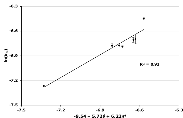
Figure 5. The relationship between the natural logarithm of the rate constant and a combination of the \beta and \pi^* Kamlet–Taft parameters for the reaction of the galactose 1 for each of the ionic liquids 3–9 at \chi ca. 0.02. Uncertainties are calculated from the standard deviation of triplicate measurements and transformed on calculating the natural logarithm.
