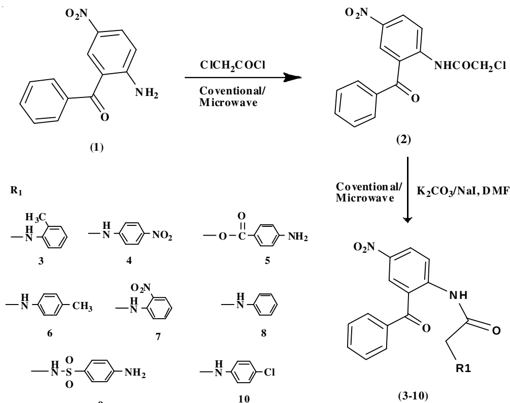
Scheme-I: Synthesis of 2-amino-5-nitro-benzophenone derivatives (3-10)
