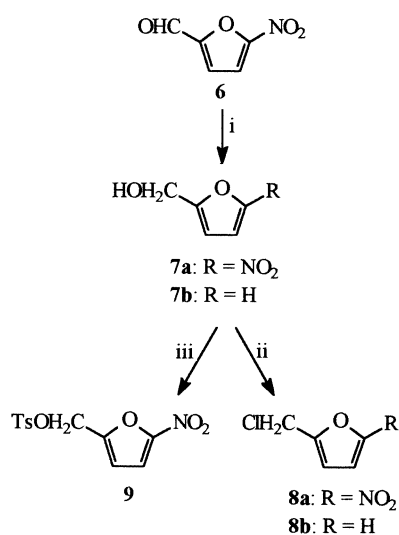
Scheme 2 Synthesis of electrophilic (nitro)furan-2-ylmethyl reagents 8a,b and 9 . Reagents: i, Al(OPr) 3 , Pr t OH; ii, SOCl 2 , pyridine, CHCl 3 ; iii, TsCl, KOH, THF.
