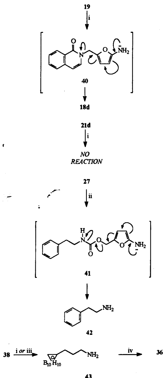
Scheme 7 Reductively activated release of isoquinolinone 18d and amines 42 and 43 from nitrofuranyl methyl ether 19 and carbamates 27 and 38 , respectively. Reagents: i, \text{NaBH}_4 , Pd-C, \text{PrOH} , water; ii, \text{NaBH}_4 , Pd-C, MeOH, water; iii, \text{SnCl}_2 , HCl, water; iv, ZCl, \text{Et}_3\text{N} , 4-pyrrolidinylpyridine, \text{CH}_2\text{Cl}_2 .
