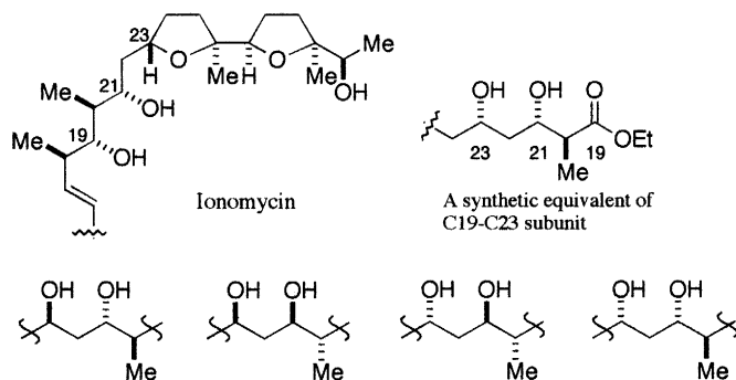
Fig. 1. Synthetic targets as enantiopure subunit
