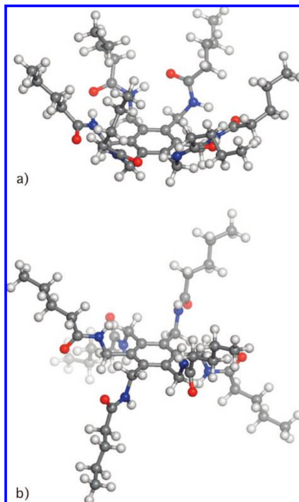
FIGURE 2. DFT-optimized views of truncated 5 13 in the (a) bowl and (b) up/down conformations.
