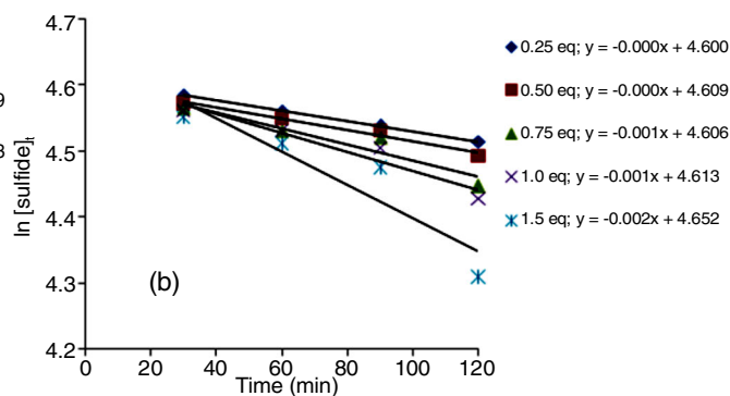
Fig. 8. First order kinetics: variation of oxidant over (a) MB-BP catalyst and (b) MoO 3 -BP catalyst
