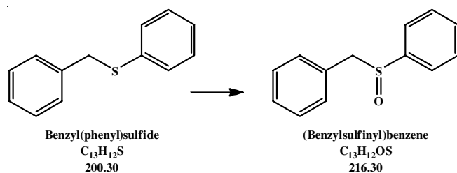
Scheme-I: Oxidation of sulfide to sulfoxide
