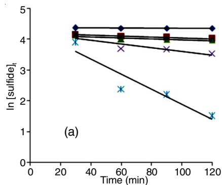
Fig. 8. First order kinetics: variation of oxidant over (a) MB-BP catalyst and (b) MoO 3 -BP catalyst
