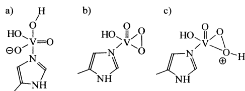
Scheme 1. The active centers of vanadate-dependent haloperoxidases from: (a) native A. nodosum bromoperoxidase, (b) the peroxo form of C. inaequalis chloroperoxidase, and (c) the hydroperoxo intermediate proposed for the A. nodosum peroxidase.
