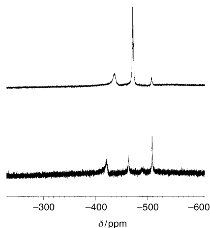
Figure 8. ^{51}\text{V} NMR spectra of 8 dissolved in \text{CDCl}_3 at 273 K, treated with CHP (bottom), and of \text{VO}(\text{OiPr})_3 + \text{H}_2\text{L4} + \text{CHP} (top). The signal indicated at -510 belongs to the peroxo complex [\text{VO}(\text{O}_2\text{R})\text{L4}] , and the two low-field signals to [\text{VO}(\text{OMe})\text{L4}] ( 8 ) and [\text{VO}(\text{OiPr})\text{L4}] , respectively.
