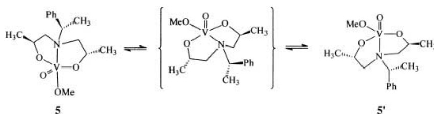
Scheme 4. Equilibrium between the two isomers 5 and 5' .
