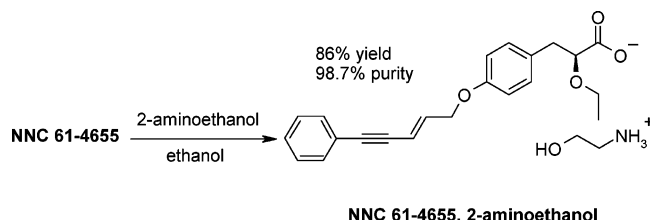
Scheme 5. Scaled GMP-kilo-laboratory synthesis of the salt NNC 61-4655, 2-aminoethanol
