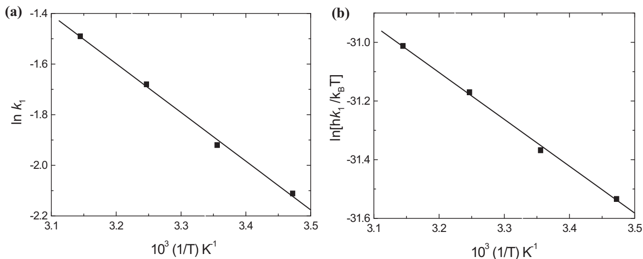
Fig. 9. (a) Arrhenius and (b) Eyring graphs of k_1 in the reduction of tellurite ion by flucloxacillin in \text{H}_2\text{SO}_4 solution. [\text{Flx}] = 5.0 \times 10^{-4} , [\text{Te}^{\text{IV}}] = 6.0 \times 10^{-3} and I = 2.0 \text{ mol dm}^{-3} .
