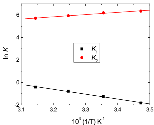
Fig. 10. Van't Hoff graphs of K_1 and K_2 in the reduction of tellurite ion by flucloxacillin in \text{H}_2\text{SO}_4 solution. [\text{Flx}] = 5.0 \times 10^{-4} , [\text{Te}^{\text{IV}}] = 6.0 \times 10^{-3} and I = 2.0 \text{ mol dm}^{-3} .
