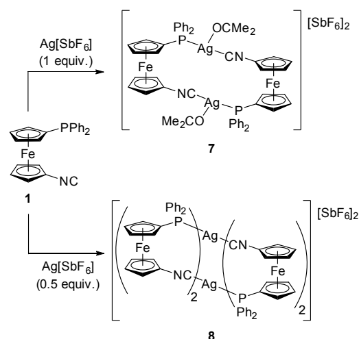
Scheme 5. Synthesis of Ag(I)- 1 complexes from Ag[SbF 6 ].
