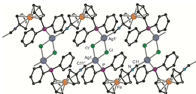
Figure 4. A section of the infinite polymeric array in the structure of 6 . For clarity, all H atoms and the less populated position of the disordered silver(I) ion were omitted. Coordination geometry parameters (in Å and deg): Ag1–P 2.4529(7), Ag1–C11 2.164(3), Ag1–Cl 2.6428(7), Ag1–Cl' 2.6358(8), P–Ag1–C11 117.71(7), P–Ag1–Cl 111.46(2), P–Ag1–Cl' 103.46(2), C11''–Ag1–Cl 110.35(7), C11''–Ag1–Cl' 120.30(8), Ag1–Cl–Ag1' 89.76(2), Cl–Ag1–Cl' 90.24(2).
