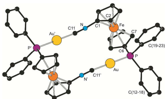
Figure 8. View of the complex cation in the structure of 11a ·2Me 2 CO. Hydrogen atoms, the counter anions and solvent molecules are omitted for clarity. Selected distances and angles (in Å and deg): Au-P 2.2821(9), Au-C11' 2.008(4), P-Au-C11' 175.8(1)^\circ , Au-C11'-N' 174.3(4)^\circ , N-C11 1.135(5), C1-C11-N 173.4(4)^\circ . The primed atoms are generated by crystallographic inversion.
