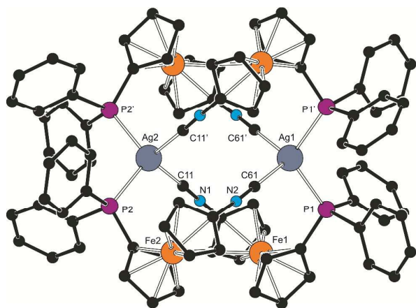
Figure 6. View of the complex cation in the structure of 8 ·3Me 2 CO. The hydrogen atoms were omitted for clarity. Coordination geometry parameters (in Å and deg): Ag1-P1 2.5376(9), Ag1-C61 2.264(3), Ag2-P2 2.5017(7), Ag2-C11 2.205(4), P1-Ag1-P1' 115.88(3), P1-Ag1-C61 103.35(9), P1-Ag1-C61' 112.44(9), C61-Ag1-C61' 109.5(1), P2-Ag2-P2' 109.65(2), P2-Ag2-C11 106.1(1), P2-Ag2-C11' 112.61(7), C11-Ag2-C11' 110.0(1), Ag2-C11-N1 177.9(3), N1-C11 1.150(5), C1-N1-C11 179.0(3), Ag1-C61-N2 178.5(3), N2-C61 1.148(3), C51-N2-C61 176.9(3). The prime-labeled atoms are generated by a crystallographic two-fold axis.
