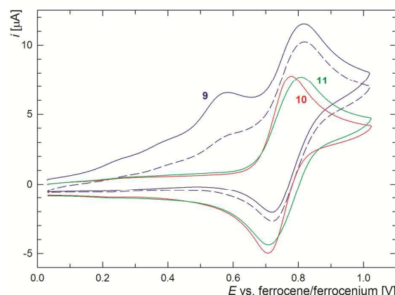
Figure 10. Cyclic voltammograms of complexes 9 (blue, the second scan is shown as a dashed line), 10 (red) and 11a (green) as recorded with a glassy carbon disc electrode in \text{CH}_2\text{Cl}_2 (scan rate 0.1 \text{ V s}^{-1} ).
