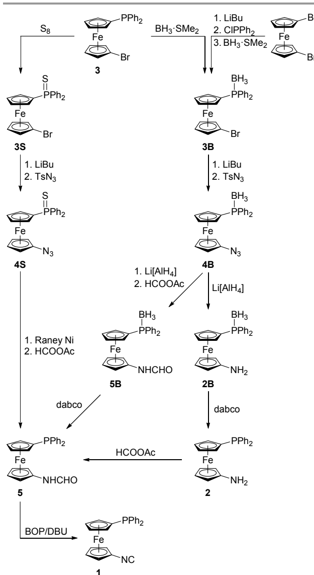
Scheme 3. Alternative syntheses of 1 exploiting different P-protected intermediates. Legend: \text{TsN}_3 = 4-toluenesulfonyl azide, BOP = (benzotriazol-1-yloxy)tris(dimethylamino)phosphonium hexafluorophosphate, dabco = 1,4-diazabicyclo[2.2.2]octane, DBU = 1,8-diazabicyclo(5.4.0)undec-7-ene.
