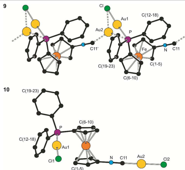
Figure 7. Simplified views of the crystal structures of 9 (top) and 10 (bottom). Selected data for 9 (in Å and deg): Au1-P 2.2298(7), Au1-Cl 2.2896(8), Au2-P 2.533(6), Au2-Cl 2.652(6), Au2-C11' 2.094(7), P-Au1-Cl 176.12(3), P-Au2-Cl 121.2(2), Au2'-N-C11
