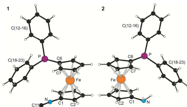
Figure 2. Molecular structures of 1 and 2.
