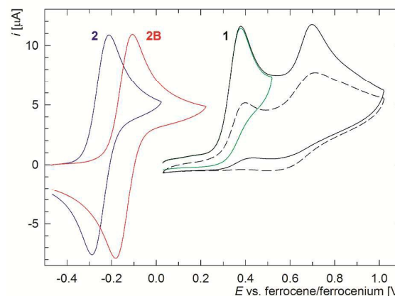
Figure 9. Cyclic voltammograms of amine 2 (blue), its \text{BH}_3 adduct 2B (red) and phosphino-isonitrile 1 (green – partial, and black – a wider scan) recorded with a glassy carbon disc electrode in \text{CH}_2\text{Cl}_2 (scan rate 0.1\text{ V s}^{-1} ). The second sweep in the voltammogram of 1 is distinguished by a dashed line.
