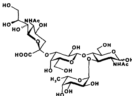
Figure 1: sialyl Lewis X
