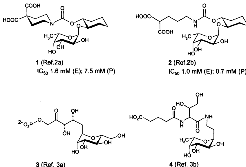
Figure 2: Designated sLe X mimetics and their IC_{50} [mM] values determined in a cell-based assay. The comparable data for sLe X are 1.5 mM (E) and 3.0 mM (P). The data published for 3 and 4 are considered to be not comparable with 1 and 2 since they were determined in cell-free assays and from samples which unfortunately had been prepared using ion exchange resins 4,5 ( IC_{50} 0.8 mM and 0.005 mM for 3 3a with E- and P-selectins, respectively, and IC_{50} 0.3 mM and 0.4 mM for 4 3b with E- and P-selectins, respectively.)
