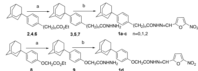
Scheme 1. Reagents and conditions: (a) hydrazine hydrate, EtOH, 3 : 160 °C, autoclave, 6 d, 81%; 5 : 130 °C, autoclave, 5 d, 85%; 7 : reflux, 2 d, 80%; 9 : reflux, 1 d, 98%; (b) 5-nitro-2-furaldehyde, EtOH, r.t., 12 h, 55-80%.
