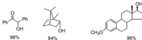
FIGURE 2 Applications of the improved odorless organosulfur reagents.
