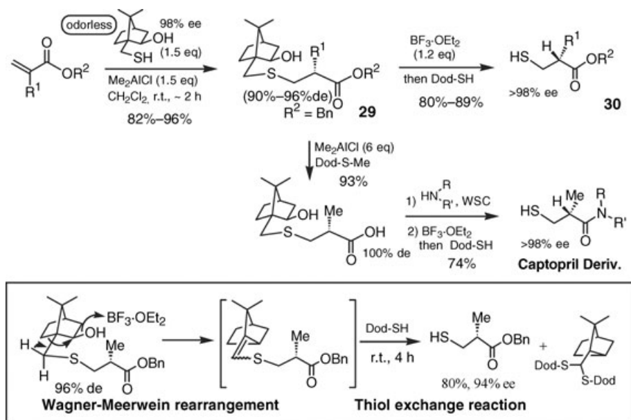
SCHEME 13 Formal asymmetric Michael addition of \text{H}_2\text{S} using odorless thiols.
