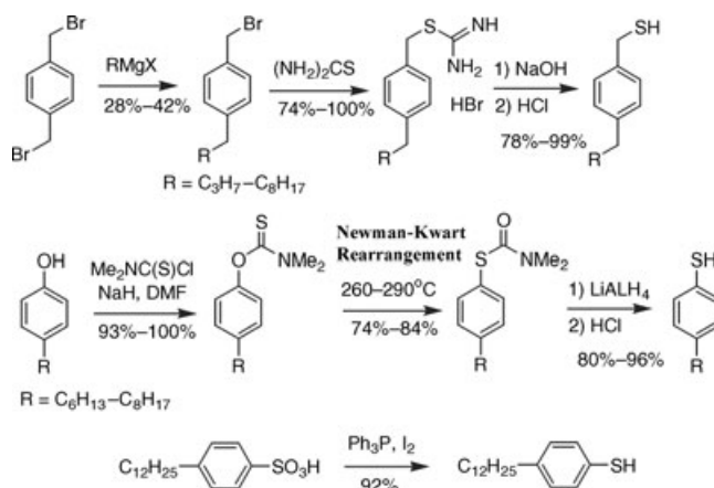
SCHEME 2 Synthesis of odorless benzyl mercaptans and benzenethiols.
