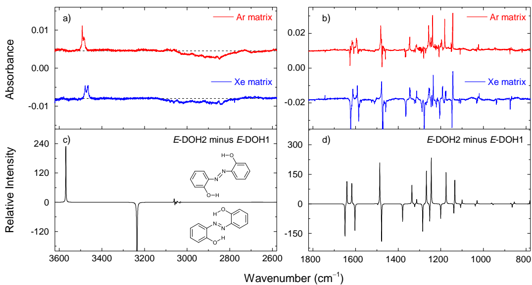
Figure 3. Changes in the experimental infrared spectra of 2,2'-dihydroxyazobenzene in argon (at 15 K) and xenon matrices (at 30 K) after irradiations at 420 nm for 4 and 2 min, respectively (panels a and b). The negative bands correspond to the consumed form (assigned to E -DOH1). The positive bands correspond to the photogenerated isomer (assigned to E -DOH2). The theoretical (M06-2X/cc-pVTZ) difference spectrum is simulated as " E -DOH2 minus E -DOH1" (panels c and d).
