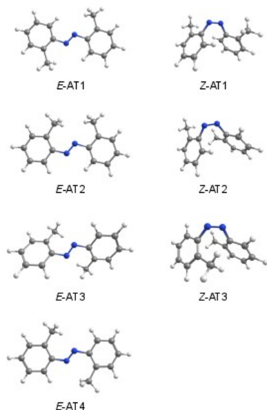
Figure 5. Isomers of 2,2'-azotoluene calculated at the M06-2X/cc-pVTZ level of theory. 42
