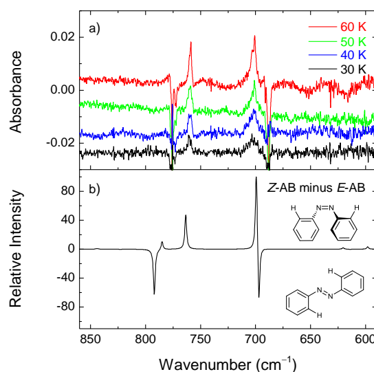
Figure 9. Changes in the experimental infrared spectrum of azobenzene in a xenon matrix after irradiation at 340 nm for 15 min at 30, 40, 50, and 60 K (panel a). The negative bands correspond to the consumed isomer ( E -AB). The positive bands correspond to the photogenerated isomer ( Z -AB). Each 340 nm irradiation was preceded by consumption of the Z form by irradiating at 420 nm for 2 min. The calculated difference spectrum (M06-2X/cc-pVTZ) is constructed as " Z -AB minus E -AB" (panel b).
