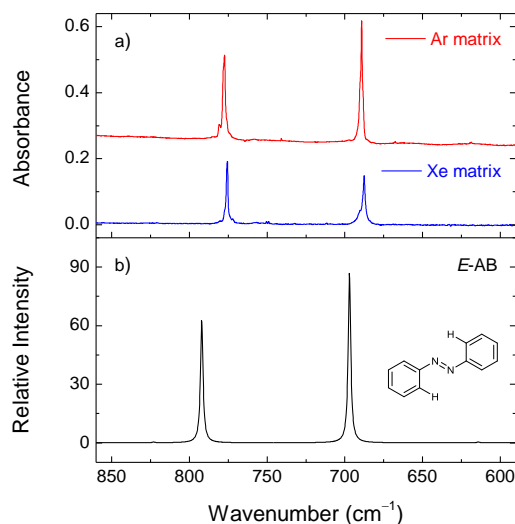
Figure 8. Selected region of the experimental infrared spectra of azobenzene isolated in xenon (30 K) and argon (15 K) matrices (panel a) and the calculated spectrum of E -AB at the M06-2X/cc-pVTZ level of theory (panel b).
