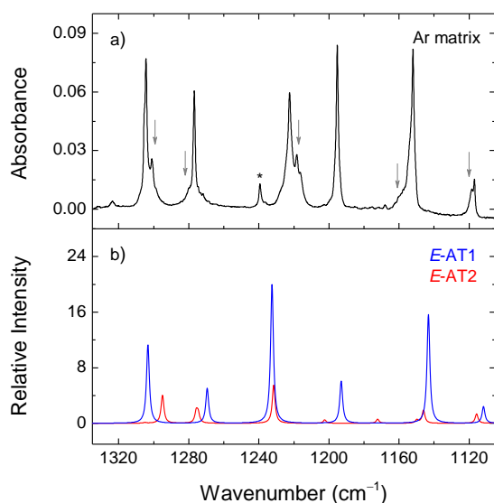
Figure 6. Selected region of the experimental infrared spectrum of 2,2'-azotoluene in an argon matrix at 15 K (panel a) and the calculated spectra of E -AT1 and E -AT2 at the M06-2X/cc-pVTZ level of theory (panel b). Arrows indicate the bands of E -AT2. The asterisk indicates a band due to traces of matrix-isolated monomeric ethanol impurity. The calculated intensities of E -AT1 and E -AT2 are scaled by 0.71 and 0.29, respectively, according to the expected gas-phase populations.
