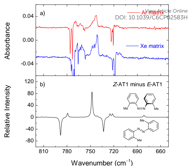
Figure 7. Changes in the experimental infrared spectrum of 2,2'-azotoluene in argon and xenon matrices after irradiation at 230 nm for 20 min (panel a). The negative bands correspond to the consumed E -AT (mainly E -AT1) form. The positive peaks correspond to the photoproduct (assigned to the Z -AT1 form). The theoretical difference spectrum (M06-2X/cc-pVTZ) was constructed as " Z -AT1 minus E -AT1" (panel b).
