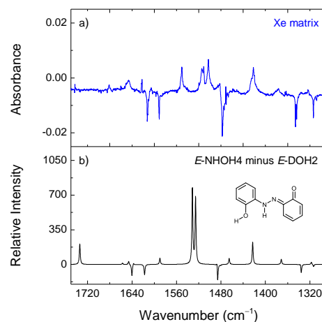
Figure 4. Changes in the experimental infrared spectrum of 2,2'-dihydroxyazobenzene in a xenon matrix at 30 K induced by irradiation at 420 nm (8 min) followed by irradiation at 323 nm (7 min; panel a). The negative absorptions correspond to E -DOH2. The positive peaks correspond to the emerging bands of a new isomeric form(s), tentatively assigned to E -NHOH4. The theoretical (M06-2X/cc-pVTZ) difference spectrum is simulated as " E -NHOH4 minus E -DOH2" (panel b).
