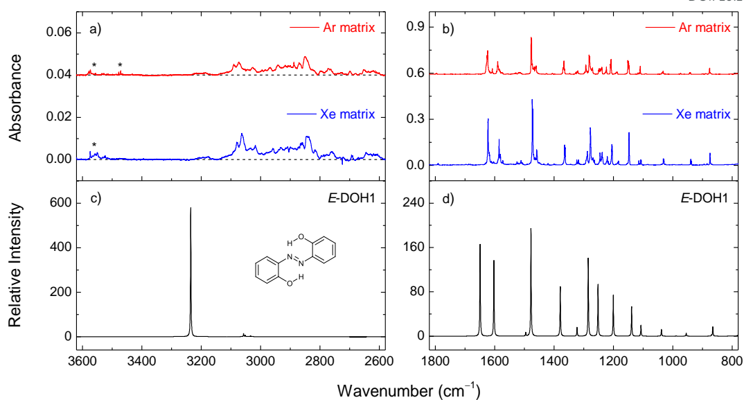
Figure 2. Selected regions of the experimental infrared spectra of 2,2'-dihydroxyazobenzene in xenon (30 K) and argon (15 K) matrices (panels a and b) and the theoretical spectrum of E -DOH1 calculated at the M06-2X/cc-pVTZ level of theory (panels c and d). The asterisks indicate the bands due to impurities.
