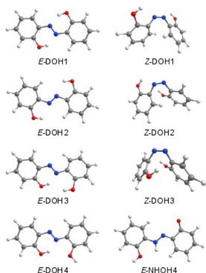
Figure 1. Structures of selected DOH and NHOH isomeric forms of 2,2'-dihydroxyazobenzene calculated at the M06-2X/cc-pVTZ level of theory. 42
