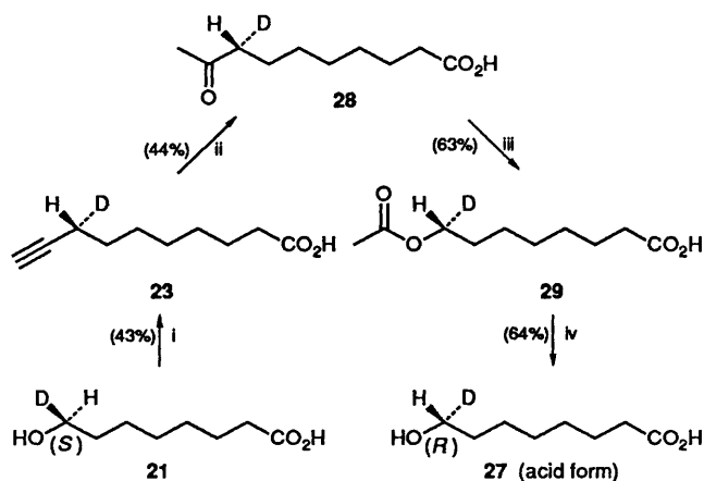
Scheme 4 Test circuit for configurational inversion by displacement using acetylide ion. Reagents and conditions: i, (a) TsCl, pyridine; (b) lithium acetylide–EDA, DMSO; ii, (a) mercury(II) acetate, aq. acetic acid; (b) NaBH 4 ; (c) PDC; iii, CF 3 CO 3 H, CH 2 Cl 2 , Na 2 HPO 4 , 0 °C; iv, EtOH, KOH.
