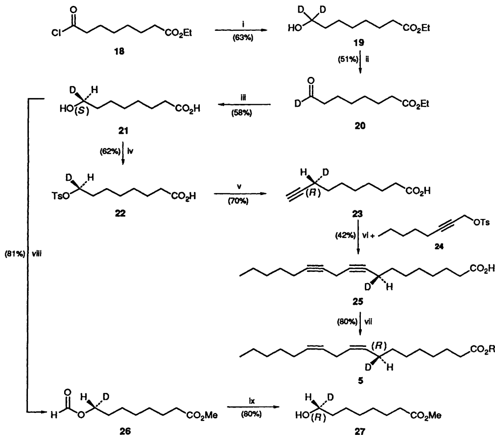
Scheme 3 Synthesis of (8 R )-[8- ^2\text{H} ]linoleic acid and Mitsunobu inversion for the enantiomeric intermediate. Reagents and conditions: i \text{NaBD}_4 , DMF-THF, 0 °C; ii, PDC, \text{CH}_2\text{Cl}_2 ; iii, bakers' yeast, glucose; iv, \text{TsCl} , pyridine; v, lithium acetylide-EDA, DMSO; vi, \text{EtMgBr} , THF, \text{CuBr}\cdot\text{DMS} ; vii, \text{H}_2 /Lindlar catalyst, quinoline, hexane; viii, (a) \text{CH}_2\text{N}_2 ; (b) DEAD, \text{PPh}_3 , \text{HCO}_2\text{H} , THF; ix, MeOH, \text{NH}_4\text{OH} .
