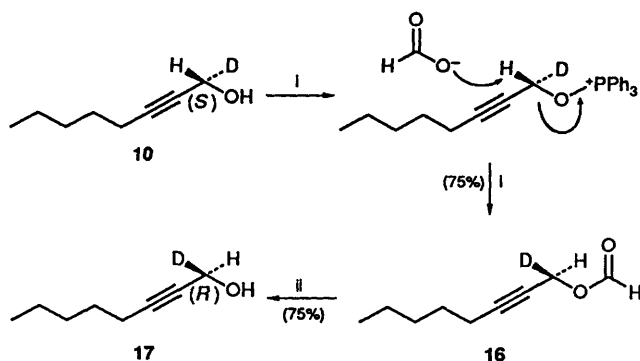
Scheme 2 (1 R )-[1- ^2\text{H} ]Oct-2-yn-1-ol by Mitsunobu inversion. Reagents: i, DEAD, \text{PPh}_3 , \text{HCO}_2\text{H} , THF; ii, MeOH, \text{NH}_4\text{OH}
