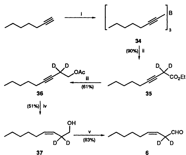
Scheme 6 Synthesis of (Z)-[2,2- ^2\text{H}_2 ]Non-3-enal. Reagents and conditions: i, (a) BuLi, THF 0 °C; (b) \text{BF}_3 \cdot \text{Et}_2\text{O} , -40 °C; ii, \text{N}_2\text{CDCO}_2\text{Et} , -40 °C, \text{D}_2\text{O} ; iii, (a) \text{LiAlH}_4 , THF; (b) \text{Ac}_2\text{O} , pyridine, DMAP; iv, (a) \text{Si}_2\text{BH} , diglyme; (b) \text{AcOH} ; (c) \text{H}_2\text{O}_2 , \text{NaOAc} ; (d) \text{LiAlH}_4 ; v, Dess–Martin periodinane, \text{CH}_2\text{Cl}_2 .
