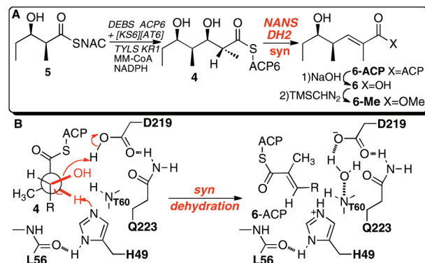
Scheme 2. (A) Stereochemistry of NANS DH2-Catalyzed Dehydration and (B) NANS DH2 Syn -Dehydration Mechanism
