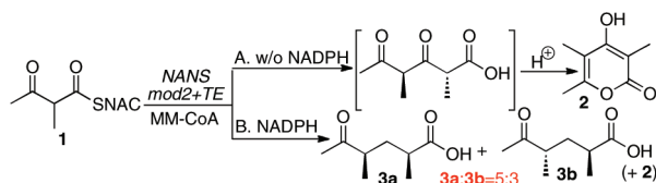
Scheme 1. Incubation of NANS Module 2+TE with 1 and Methylmalonyl-CoA (A) without NADPH and (B) with NADPH
